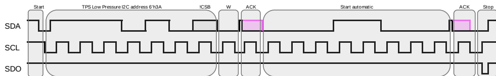
Figure 27: I2C start automatic mode command
