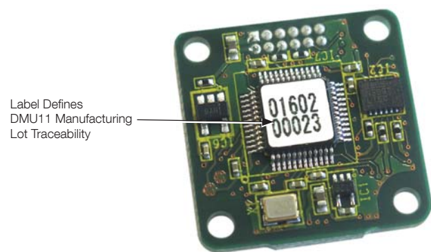
Figure 9.2 Lot Traceability
