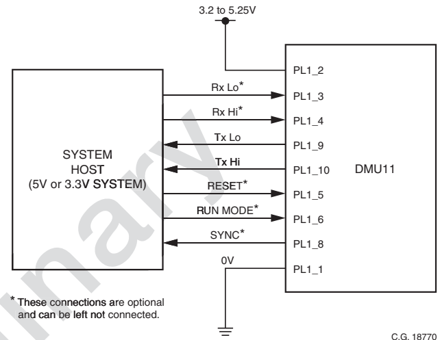
Figure 7.1 Required Connections for RS422 Communications with DMU11
