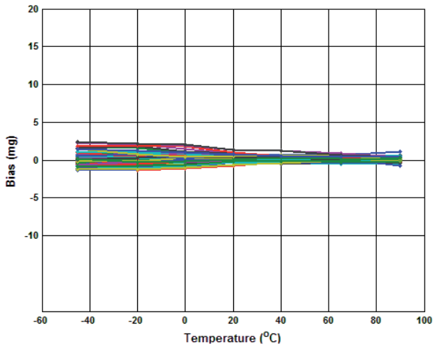
Figure 5.5 Accelerometer Bias
