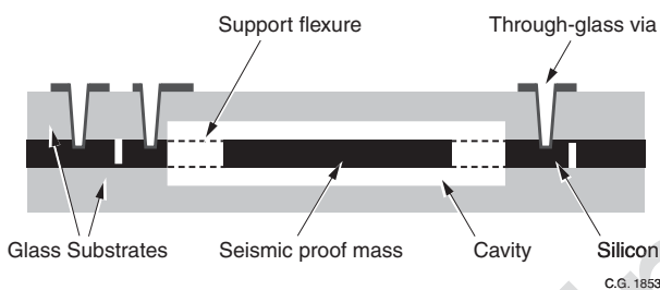
Figure 11.3 Schematic Section of the Silicon On Glass Accelerometer MEMS Wafer Sub-Assembly
