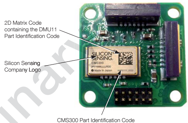
Figure 9.1 Part Identification
