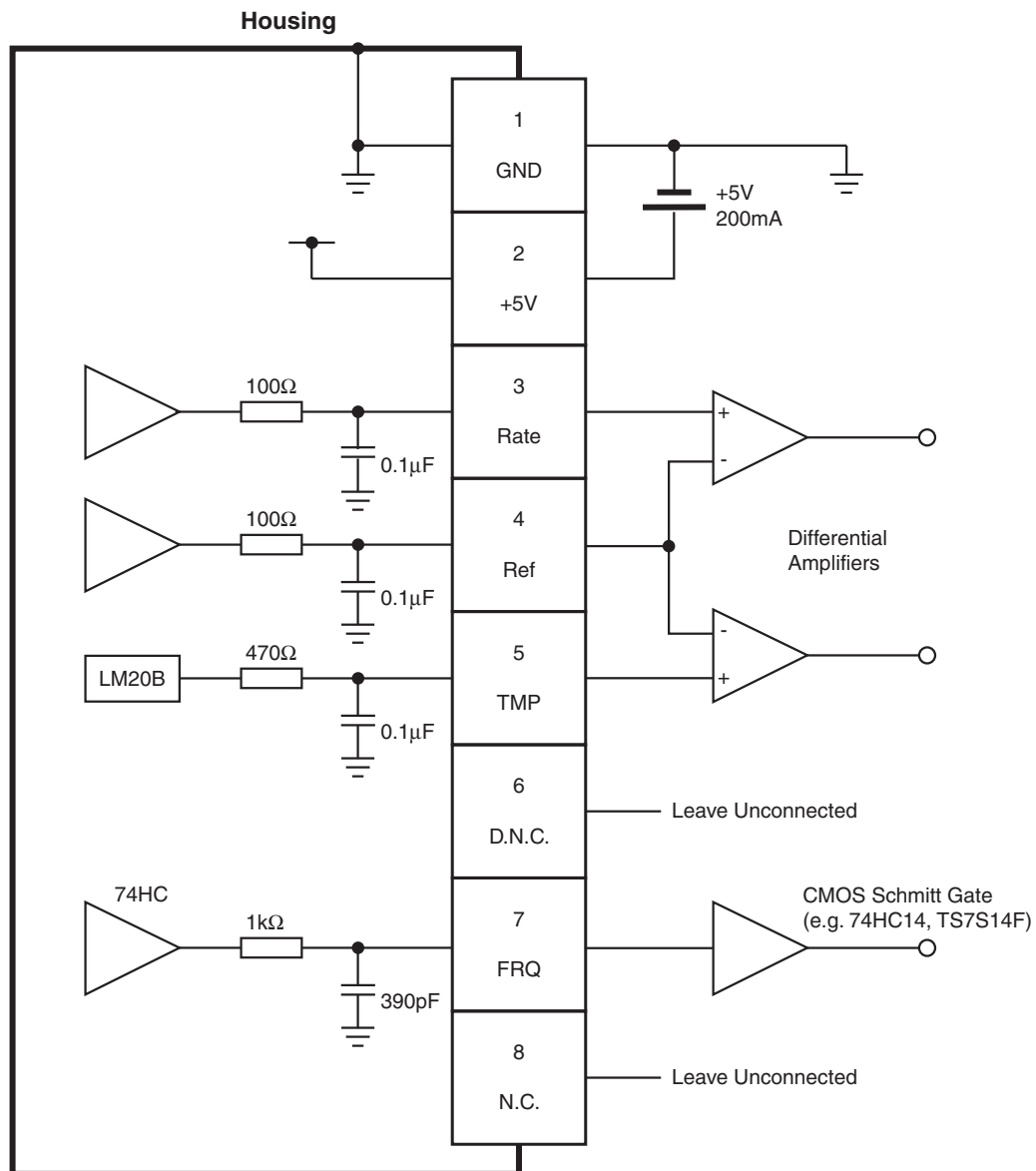
Figure 7.1 Recommended Interfacing
